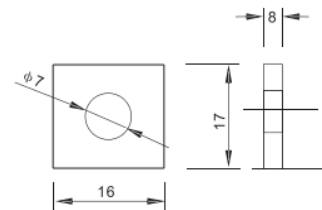
T5 terminal with M6 Nut and Bolt hardware (Stocked option)
